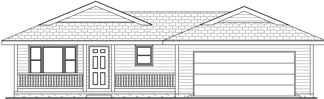
FRONT ELEVATION
