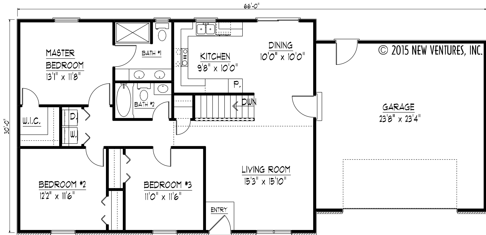
MAIN LEVEL FLOOR PLAN
